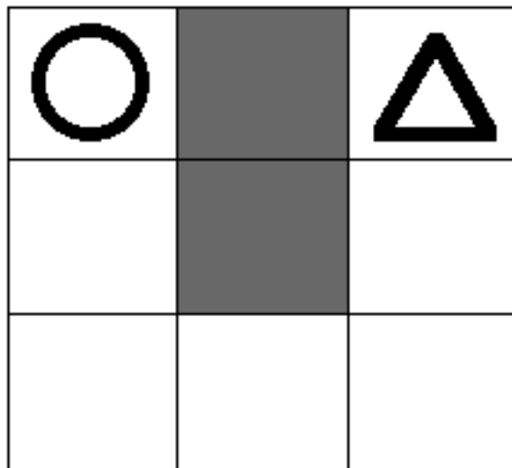
Figure 1. 2D grid.
