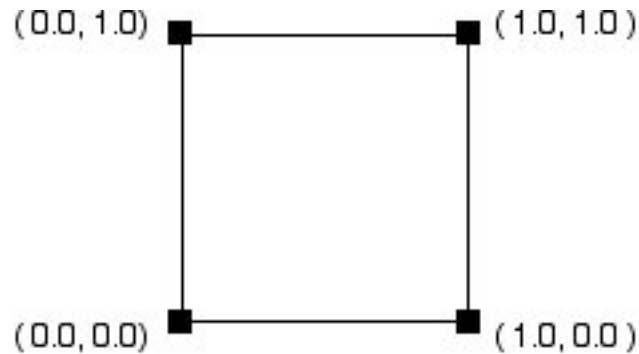
Figure 7. Texture mapping.
